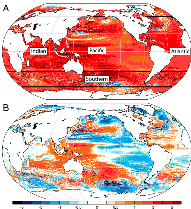
Fig. 1. Regional sea-level trends from altimetry (millimeters year -1 ) from 1993 to mid-2018 (A) based on annual averages of raw AVISO estimates ( https://www.aviso.altimetry.fr/en/my-aviso.html ) and (B) with the global mean rate of rise removed. Also shown in A are the boundaries for the Pacific, Atlantic, Indian, and Southern Oceans used for defining ocean basins as defined in this analysis.
